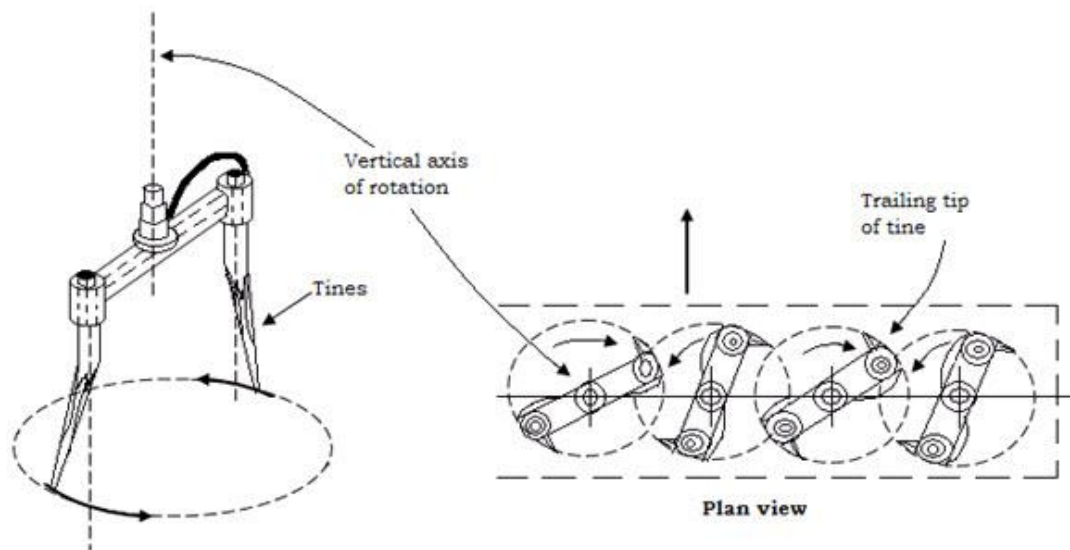
Fig. 19.2 Vertical Axis Rotary Tillers
