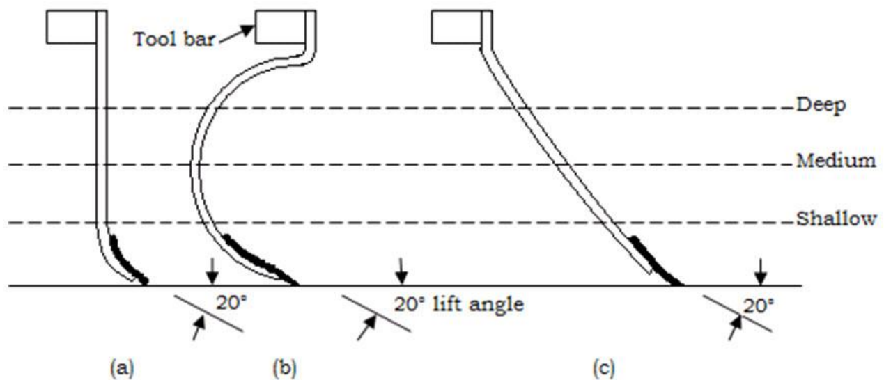
Fig. Rotation of chisel-type tool
