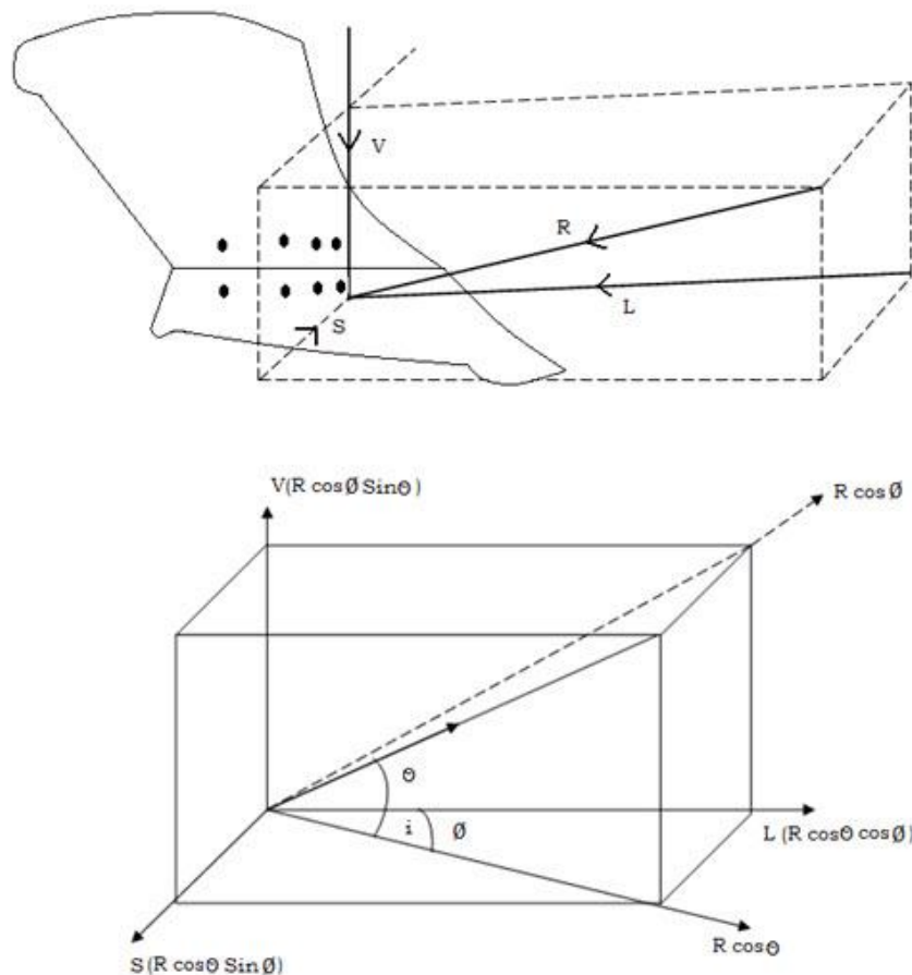
Fig.15 Forces Acting on a Tillage Tool
