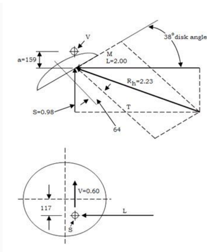
Fig. 16 (b) Horizontal Force R_h , plus Vertical Force V
