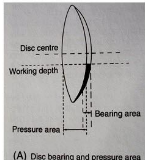
Fig. 4 Disc Bearings
