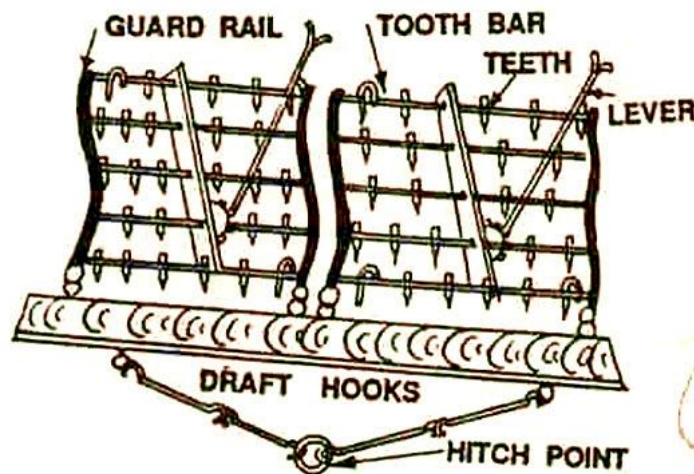
Fig.5. Spike tooth harrow
