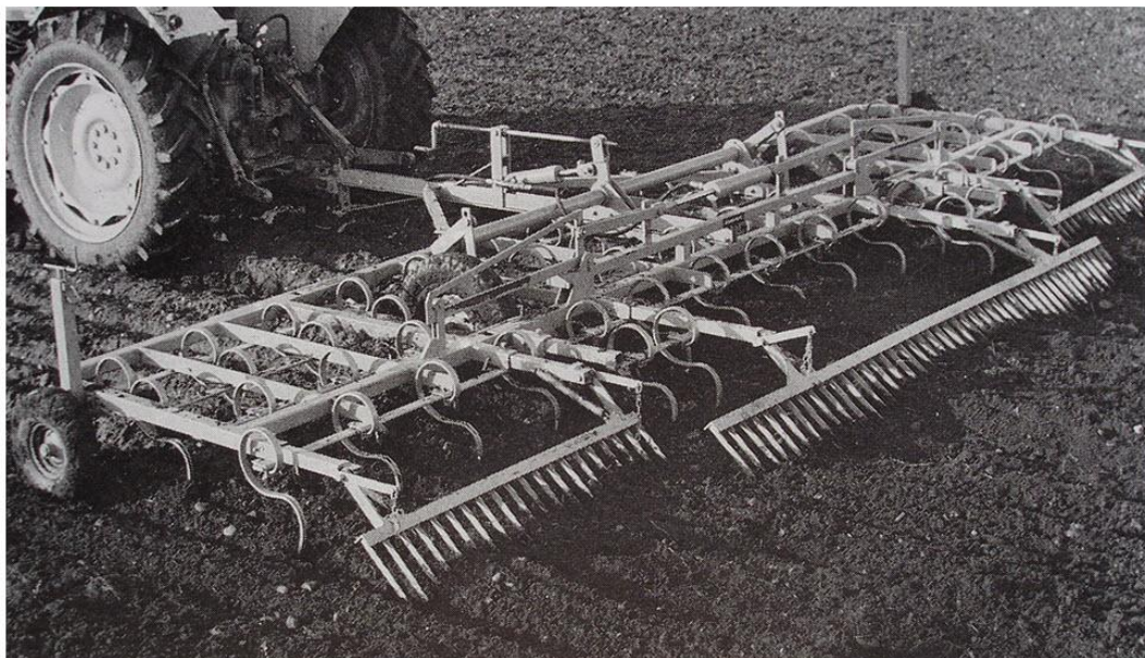
Fig. 6. Spring tined harrow combined with backward sloped crumbler
