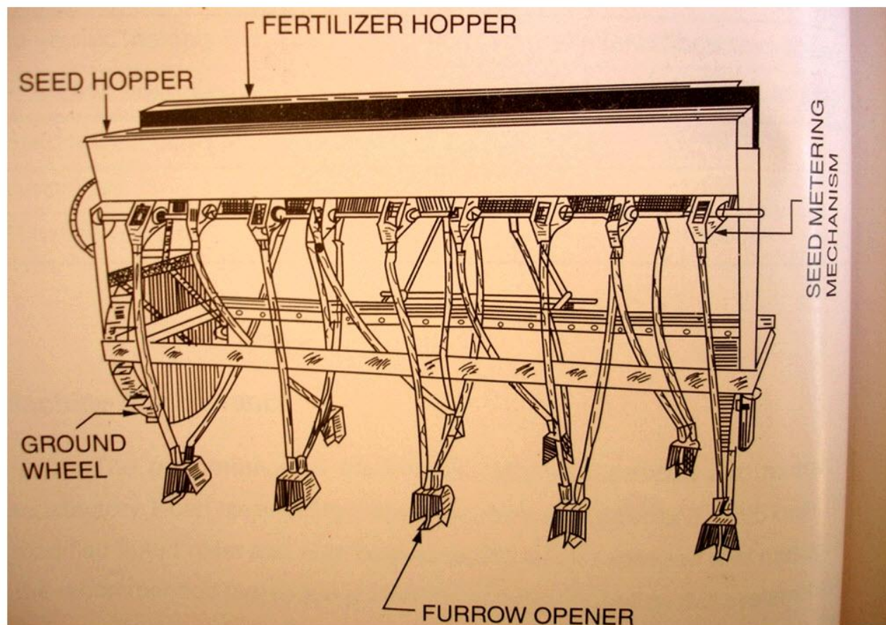
Seed Drill
