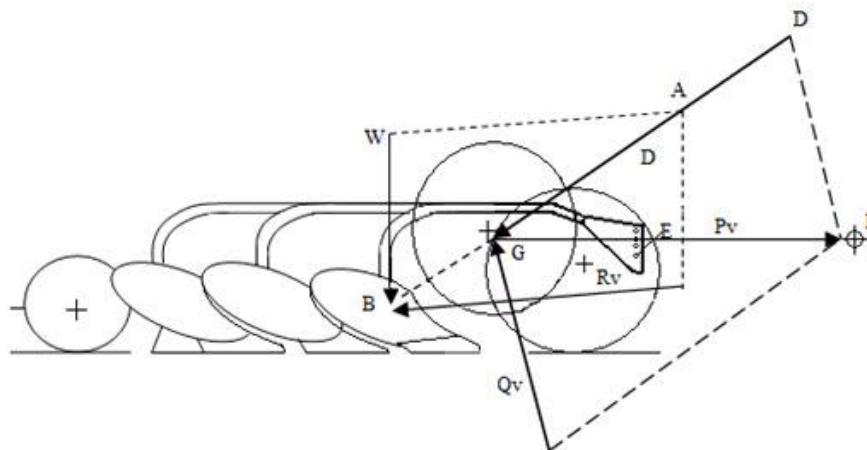
Fig. 17.4 Vertical force relation for a pull type mould board plough having support wheels and hinged pull members
