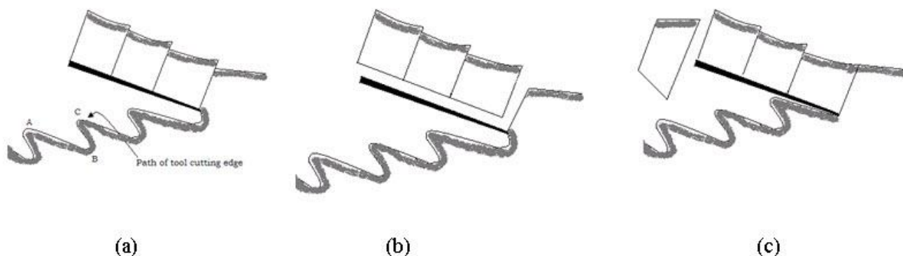
Fig. 19.1 Idealized operation of an oscillating tillage tool. (a) separation and upward acceleration of the soil, (b) soil lifted from tool by inertia at beginning of the cutting stroke and (c) end of cutting stroke
