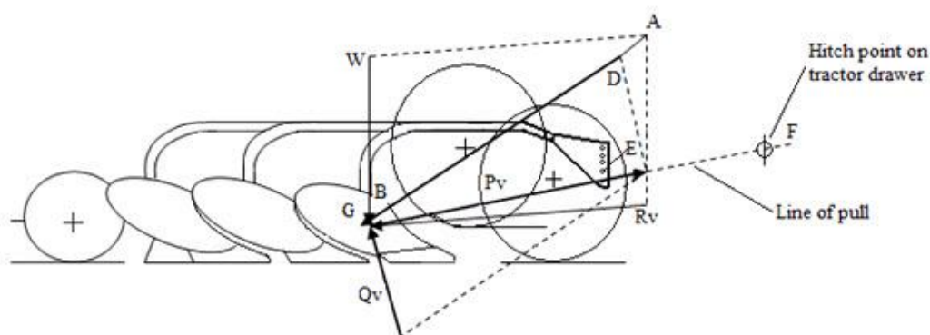
Fig. 17.3 Vertical force relation for a pull type mould board plough having support wheels and hinged pull members
