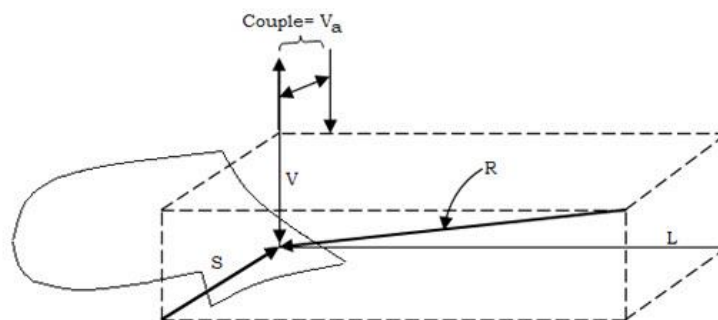
Fig. 16 (b) One force R , plus a couple V_a in a plane 1 to the line of motion.
