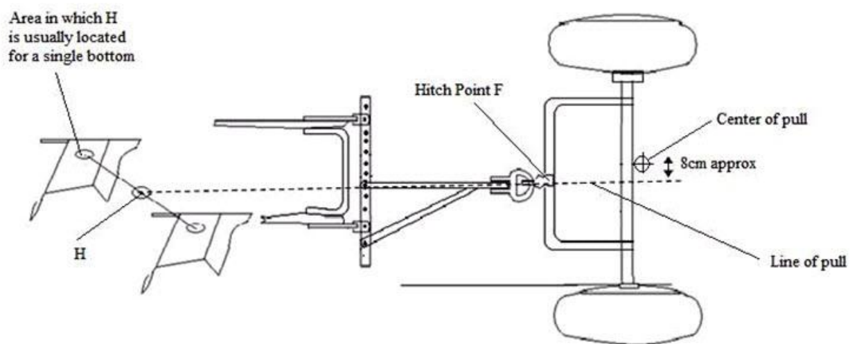
Fig. 17.1 Horizontal hitching for a mold board plow pulled by wider tractor
